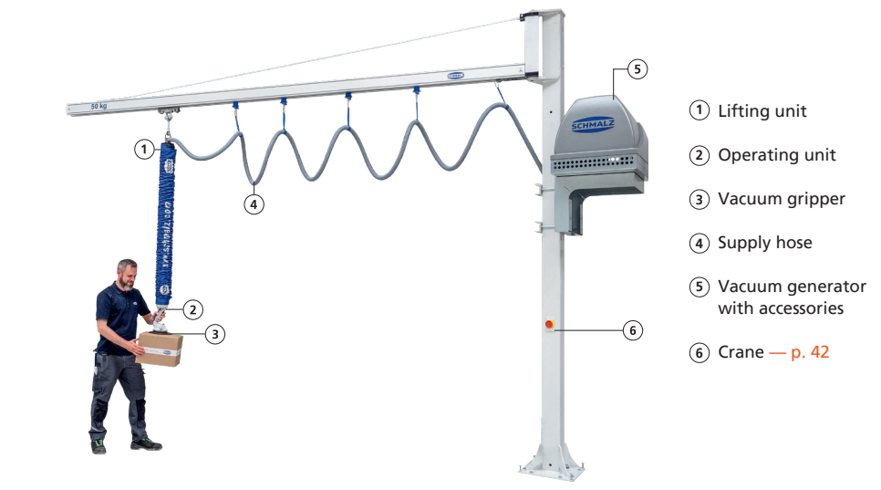
The entire system and its individual parts
