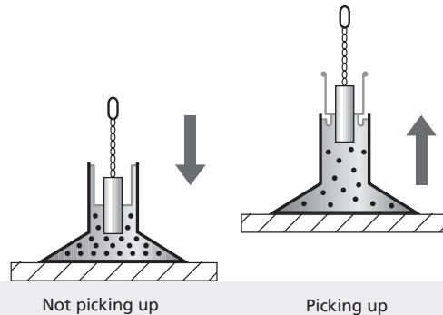
Functional principle of VacuMaster Eco
