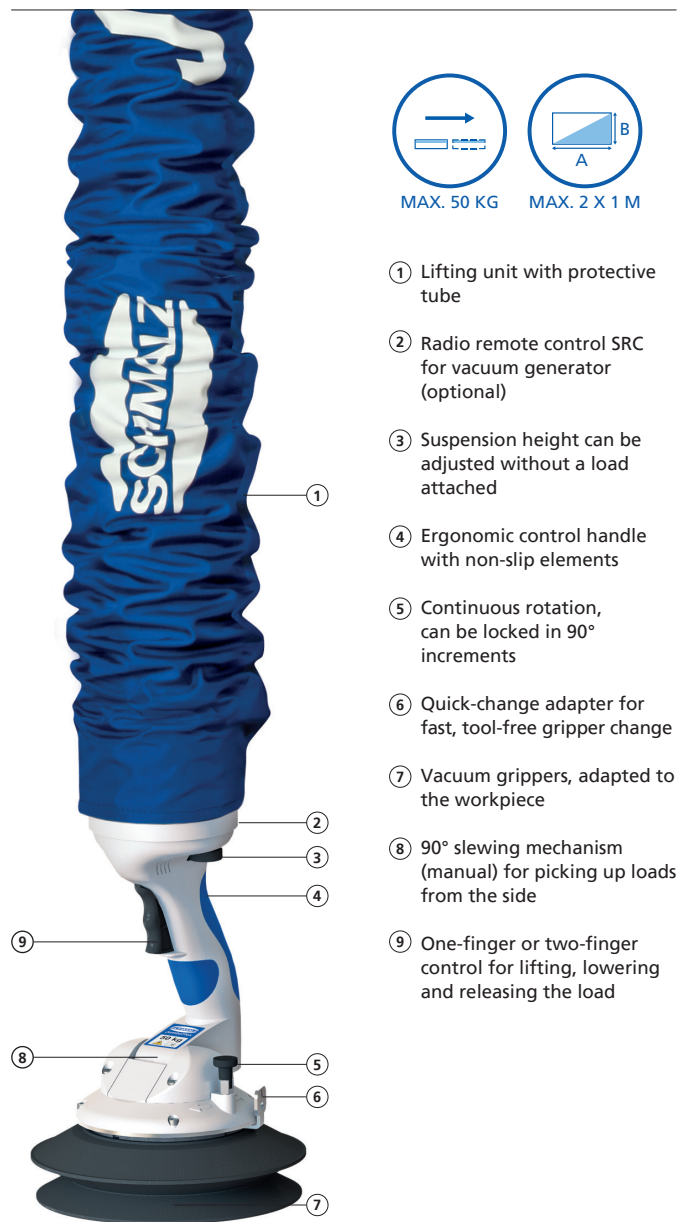
JumboFlex 50
