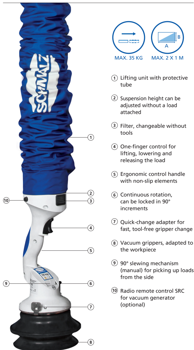
JumboFlex 35
