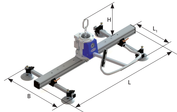
Design of VacuMaster Eco
