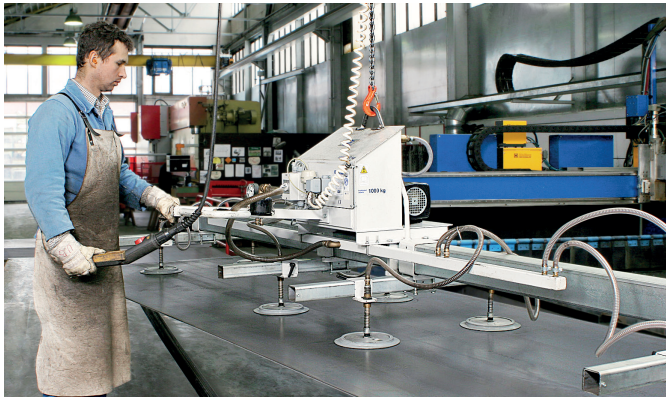
VacuMaster Vario in process of loading and unloading a laser cutting machine
