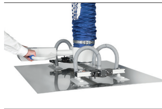
Quadruple vacuum gripper For large cardboard boxes, sheets and non-rigid pieces. The vacuum grippers can be continuously adjusted lengthwise and crossways.
