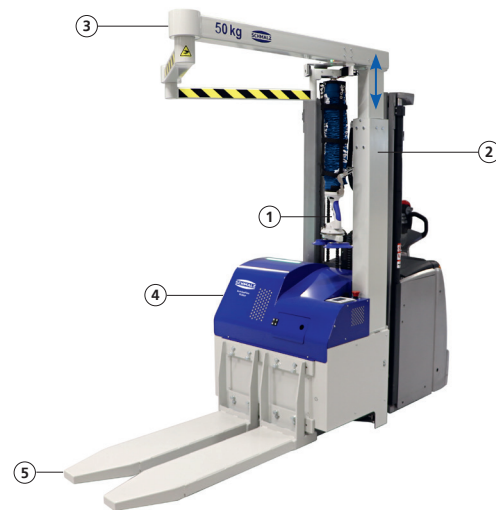
Design JumboFlex Picker
