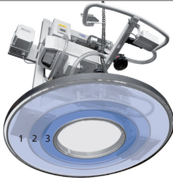
Suction plate with three separate vacuum clamps
