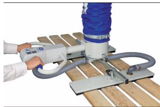
Vacuum area gripper FMP For pallets, sections or cut pieces where the vacuum gripper is not fully covered by the workpiece. The grippers can be continuously adjusted along the beam.
