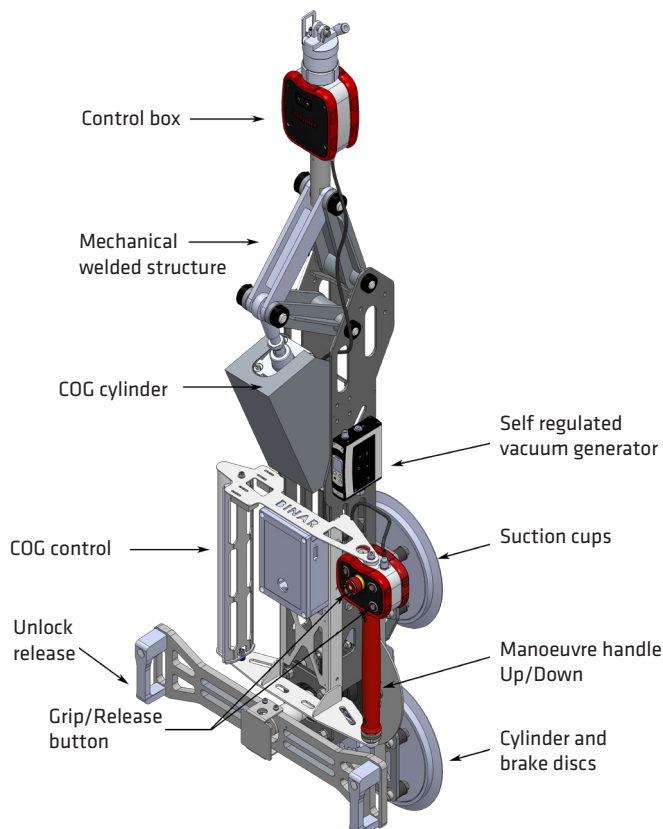
Picture showing end effector with both manual and pneumatic rotation function.
