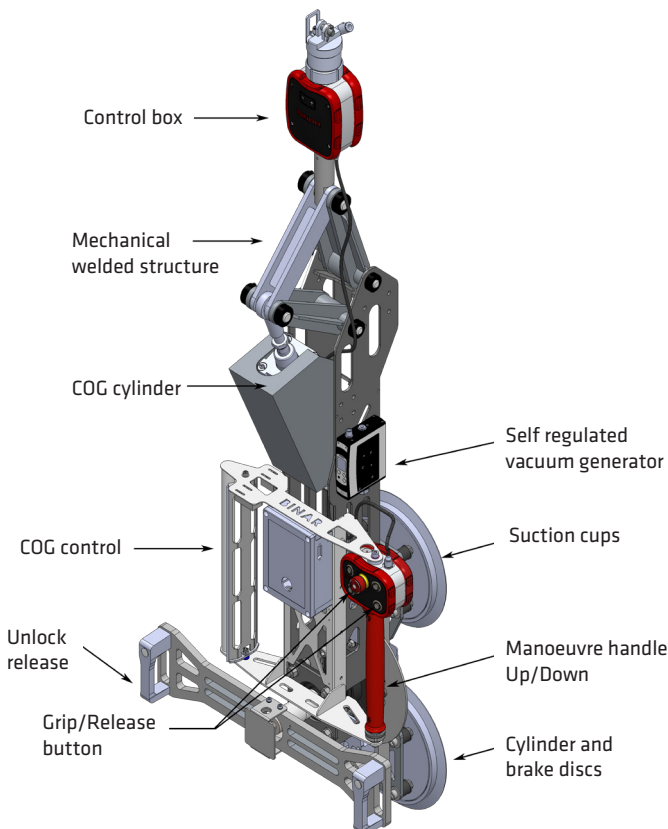
Picture showing end effector with manual rotation.
